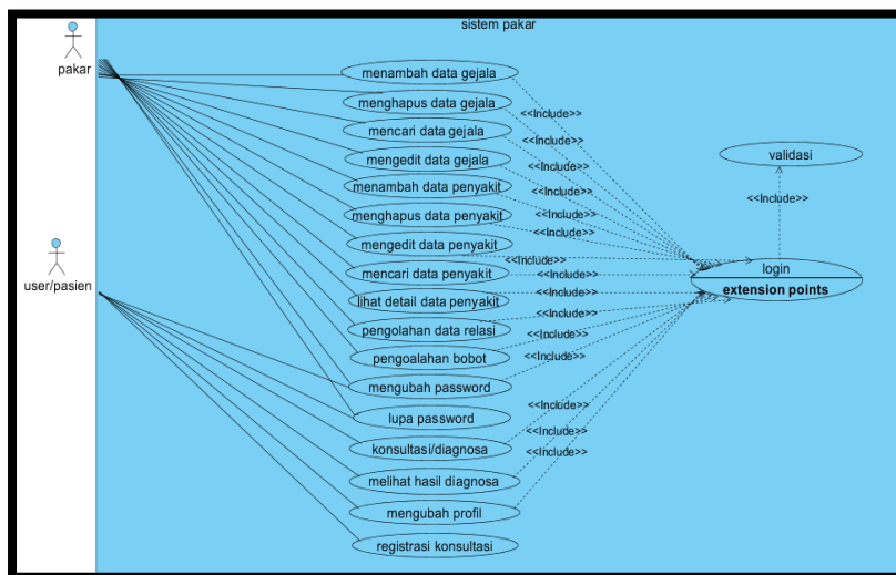
Gambar 1. Use Case Diagram Sistem Pakar
