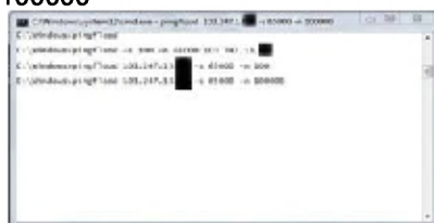
Gambar 13. Perintah pingflood
