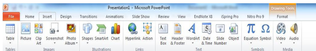
Gambar 2. Toolbox PowerPoint 2010
